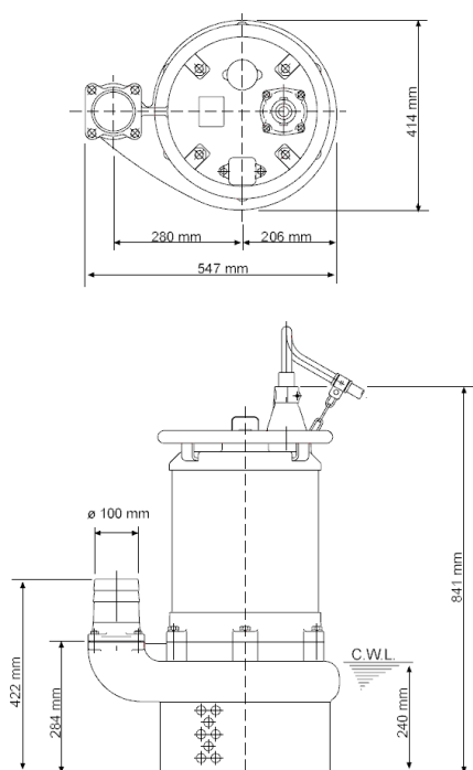
NKZ3-100H
