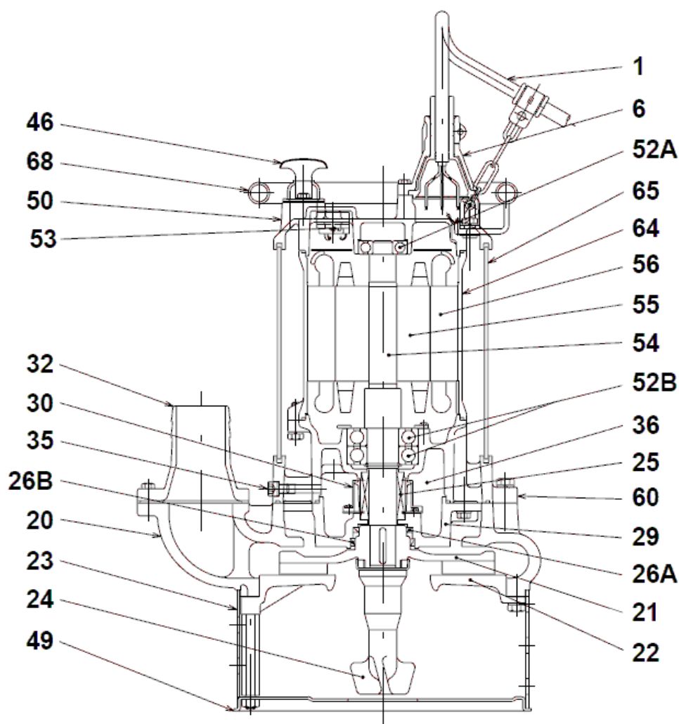
NKZ3-100H
